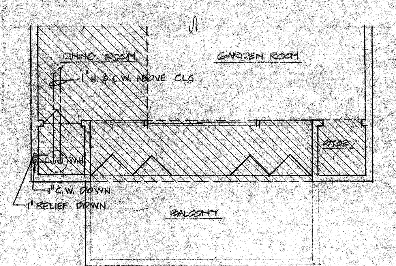
BALCONY DETAIL
