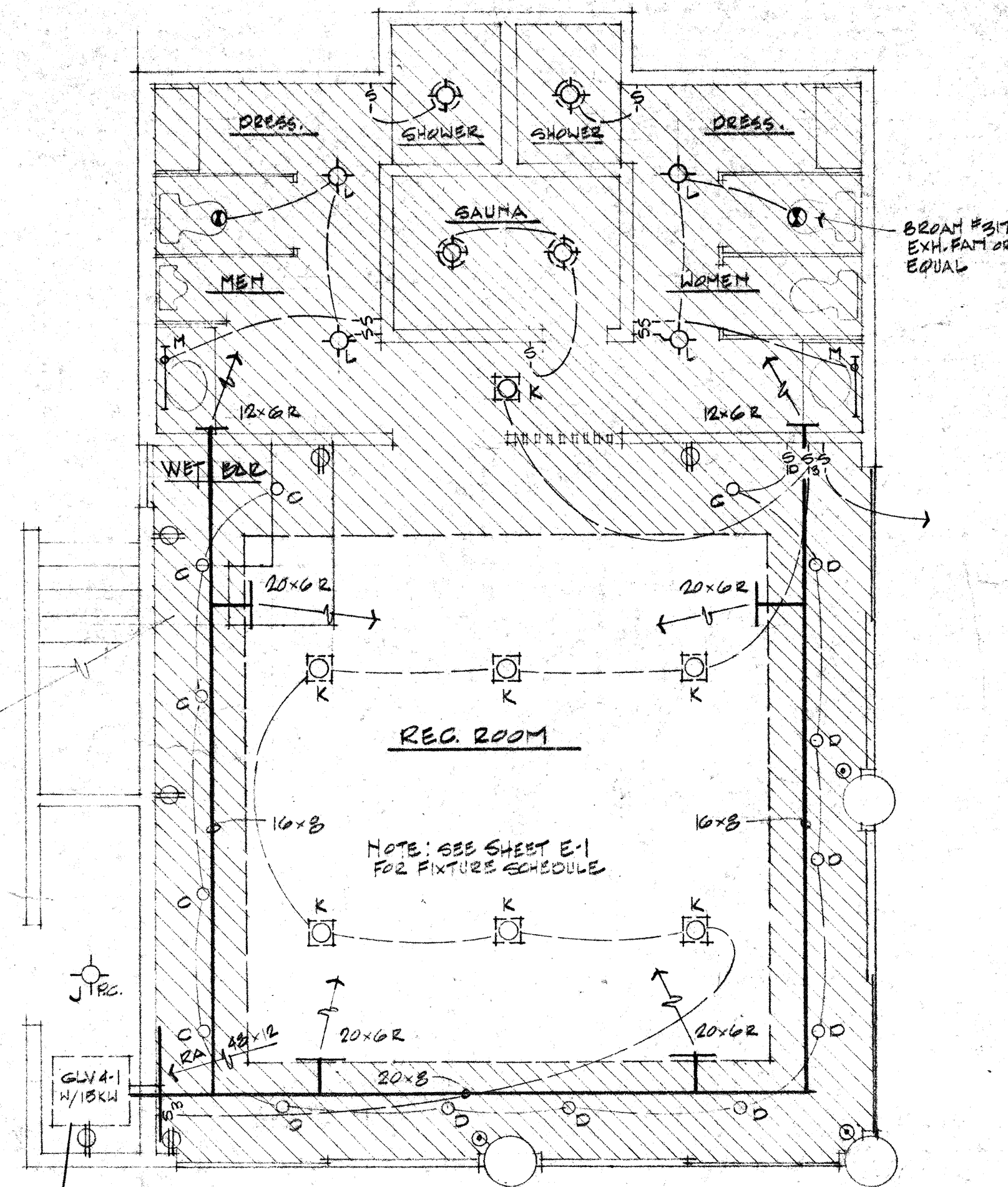
ELECTRICAL/MECHANICAL PLAN @ REC. RM. SCALE 1/4"=1'-0"
