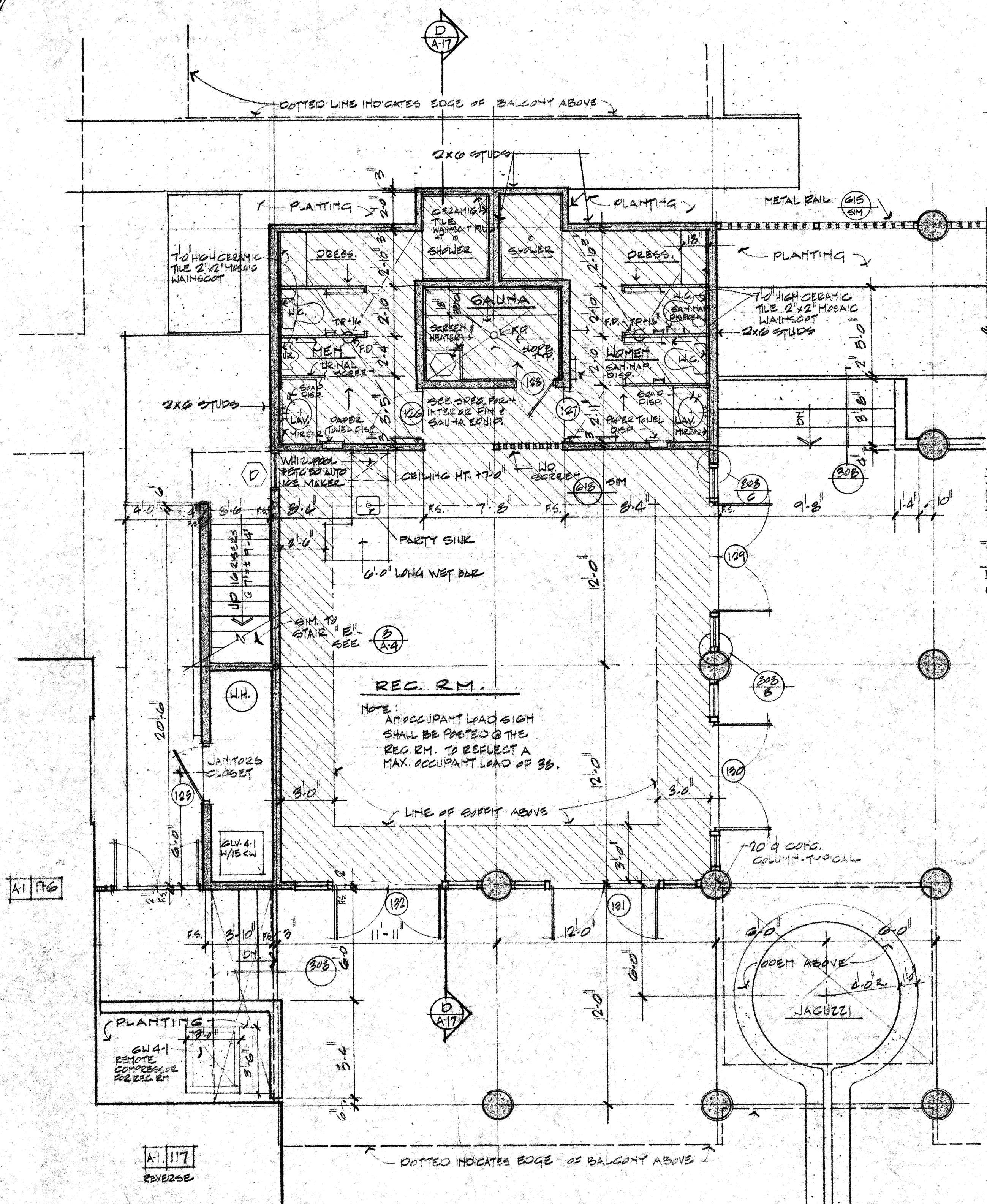
FLOOR PLAN @ REC. RM. SCALE: 1/4"=1'-0"
